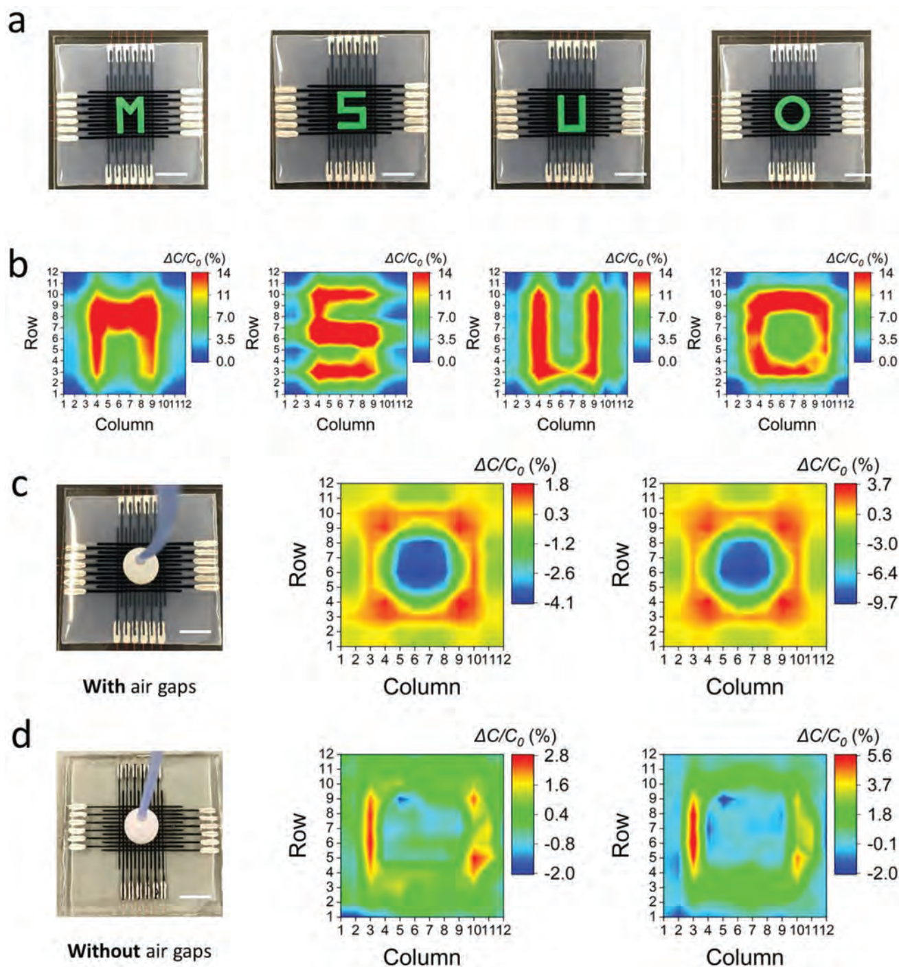
Figure 4. Spatial mapping of pressure distributions with the sensor array under both positive and negative pressures. a) Photograph of the 12 × 12 pixel sensor array with different shaped objects placed on top for pressure mapping testing. Scale bar: 2 cm. b) The corresponding distributions of the normalized capacitance change with +10 kPa pressure applied. c) Photograph of the 12 × 12 pixel sensor array with air gaps ( H = 0.5 mm, W = 1.2 mm) and the corresponding contour plots of relative change in capacitance under a negative pressure of -10 kPa (left) and -20 kPa (right). Scale bar: 2 cm. d) Photograph of the 12 × 12-pixel sensor array without an air gap and the corresponding contour plot of relative change in capacitance under a negative pressure of -10 kPa (left) and -20 kPa (right). Scale bar: 2 cm.
